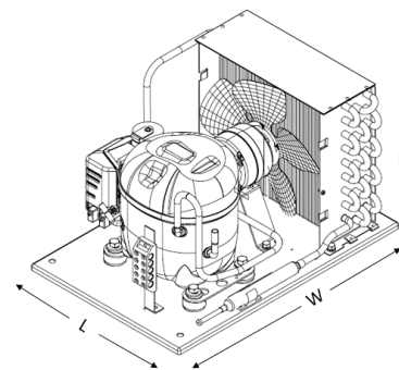
Low height Single fan: AE AE2415YGHXR AE4440YGHXR
