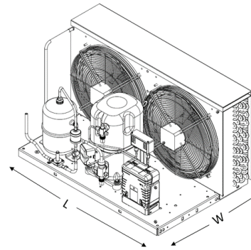
HHP Condensing Unit: AG
