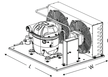
Low height Twin fan: AE AE4460YGHXR
