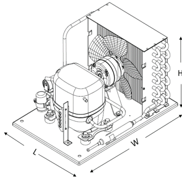
Low Height FHP : TH THK9417YJEXR THK2390YJEXR THK2411YGHXR
