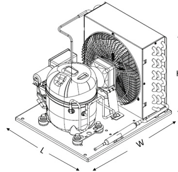
Standard FHP: AE AE4460YGHXR
