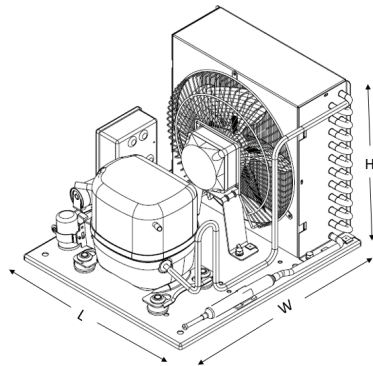
Standard FHP : TH THK9417YJEXR THK2390YJEXR
