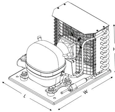
Standard FHP : TH THK1365YCGXR THK9410YCGXR THK9384YCGXR THK9414YGHXL
